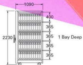
12 arch files (A4) per shelf. 1 bay 60 arch files.
