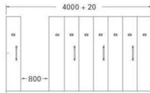
8 BAY
