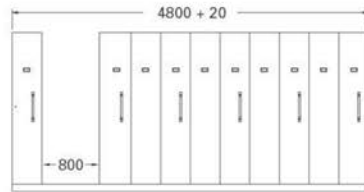
10 BAY
